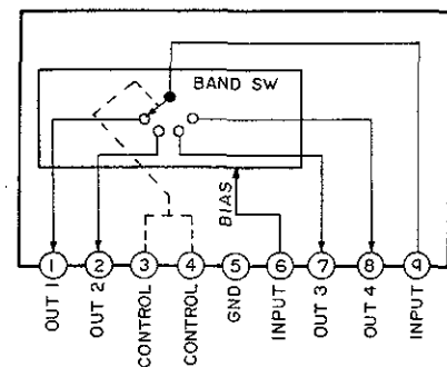
IC,LA7910
