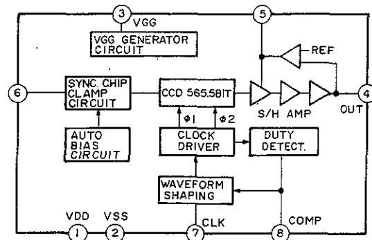
IC,LC8992
